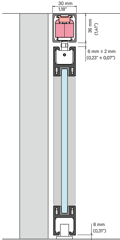
3 Perfil oculto "T" | Exposed Track | Rail visible
