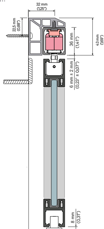
4 Perfil soporte pared 6 mm / 17 mm | Wall support profile 6 mm / 17 mm | Profil de support mural 6 mm
